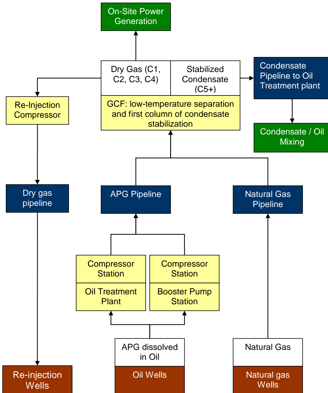
Process Flow after partial project implementation (1 st stage)
