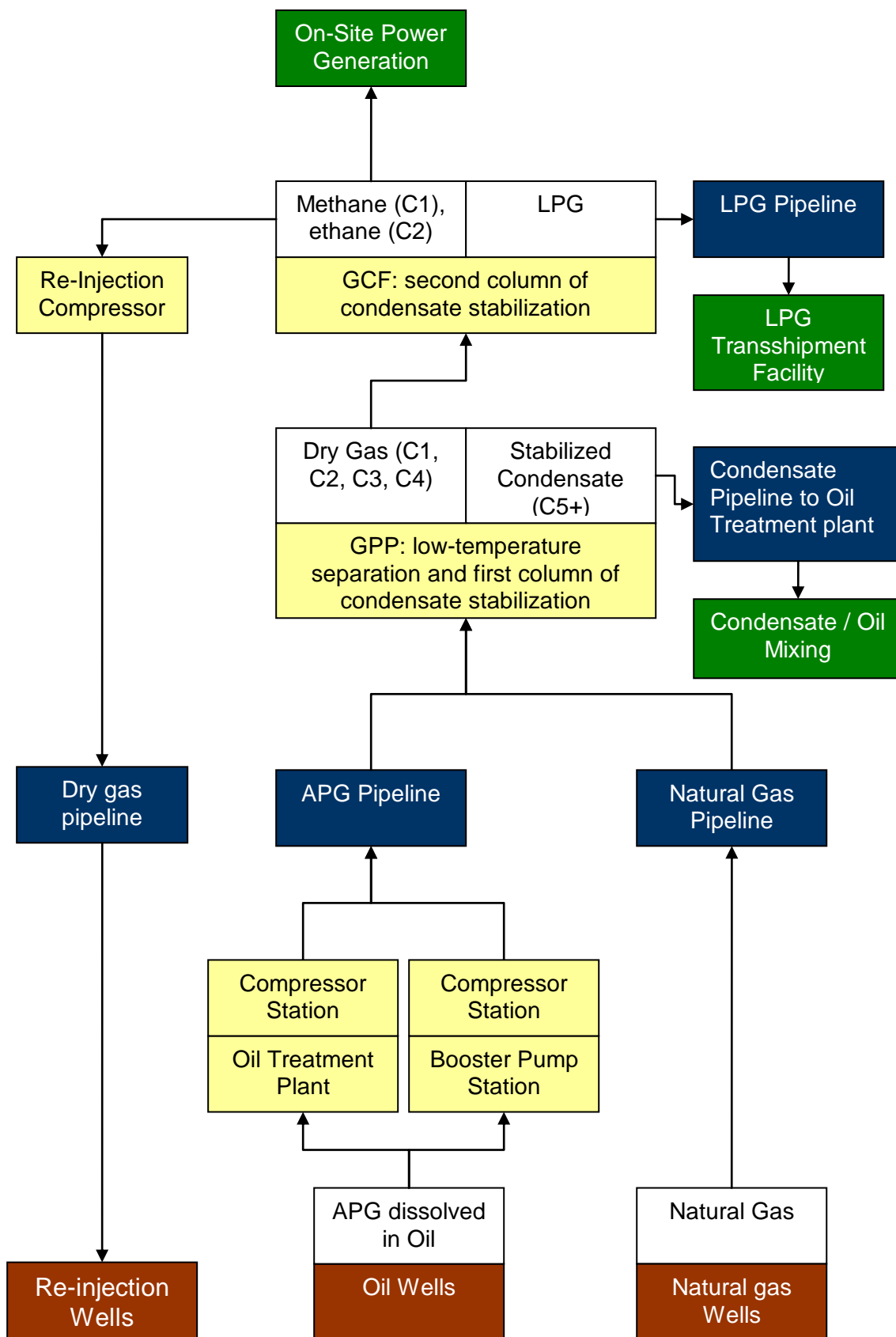
Process Flow after Project Implementation (2 nd stage)
