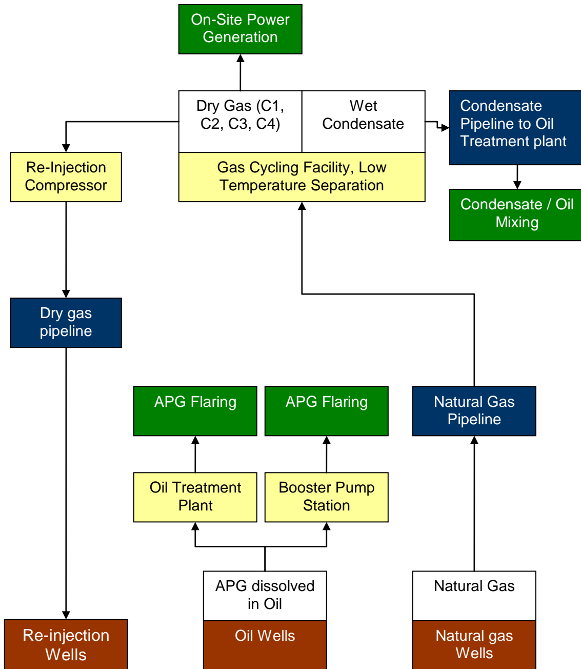
Baseline Process Flow
